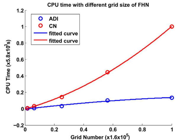
Fig. 12. The CPU time versus grid number for the FitzHugh-Nagumo model with \Delta t = 0.2 and \Delta x = \Delta y = 1 ; the total time is 1000.
