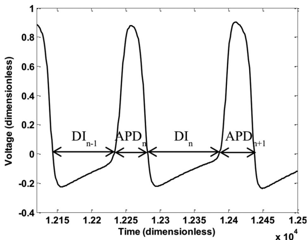
Fig. 1. Illustration of the action potential duration (APD) and the diastolic interval (DI).
