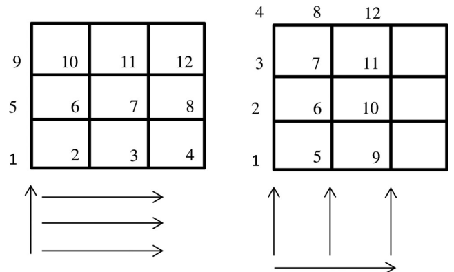
Fig. 2. The order of the grids in the alternating direction implicit method. Step 1 (left): x -direction first; step 2 (right): y -direction first.
