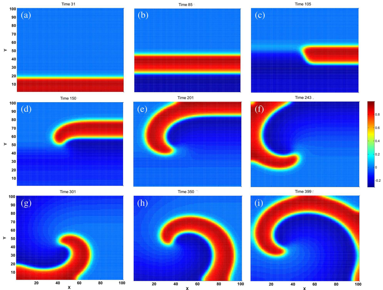
Fig. 3. Spiral wave evolution in the FitzHugh-Nagumo model computed using the alternating direction implicit method. The domain size is 100 \times 100 , \Delta x = \Delta y = 1 , and \Delta t = 0.2 . The spiral wave is shown for the first 400 time units.
