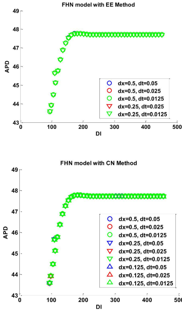
Fig. 7. There is no significant difference of the action potential duration restitution curves of the FitzHugh-Nagumo model obtained by two methods (top: explicit Euler; bottom: Crank-Nicolson) with different \Delta t and \Delta x values.
