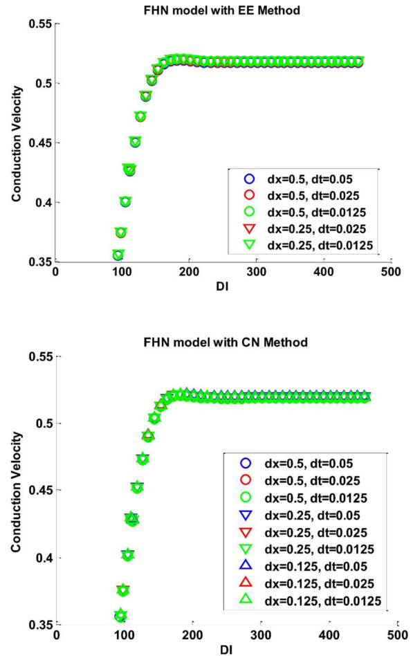
Fig. 8. There is no difference in the conduction velocity restitution curves for the FitzHugh-Nagumo model for the \Delta t and \Delta x values considered (top: explicit Euler; bottom: Crank-Nicolson).
