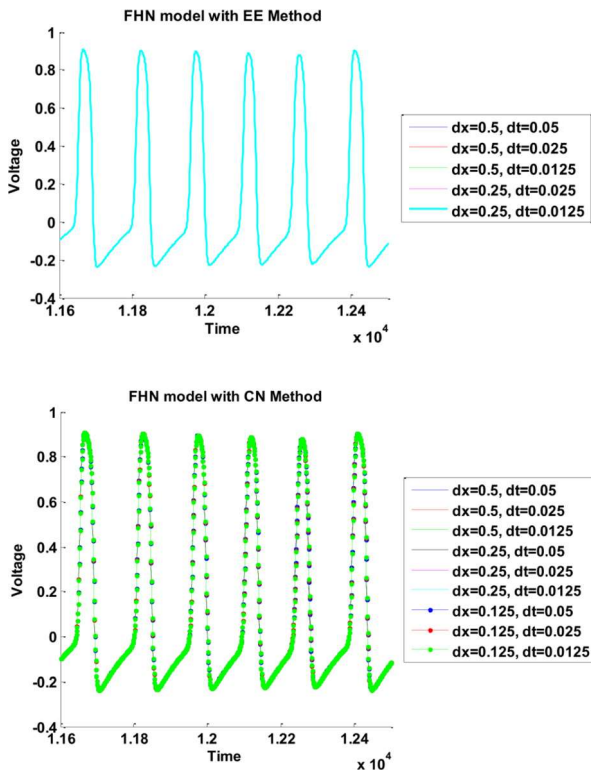
Fig. 6. The action potential of the FitzHugh-Nagumo model for different \Delta t and \Delta x values (top: explicit Euler; bottom: Crank-Nicolson). A train of stimuli is delivered with the pacing cycle length starting from 500, decreasing by 10 every beat until it reaches 50. The last ten stimuli are shown, which generate only six excitations due to conduction block. (They fail to produce a propagation because the cells are still in their refractory periods.) The resting potential is zero and the voltage is dropped below the resting potential after depolarization.
