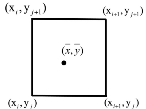
Fig. 5. Bilinear interpolation allows us to find the tip within the grid points.
