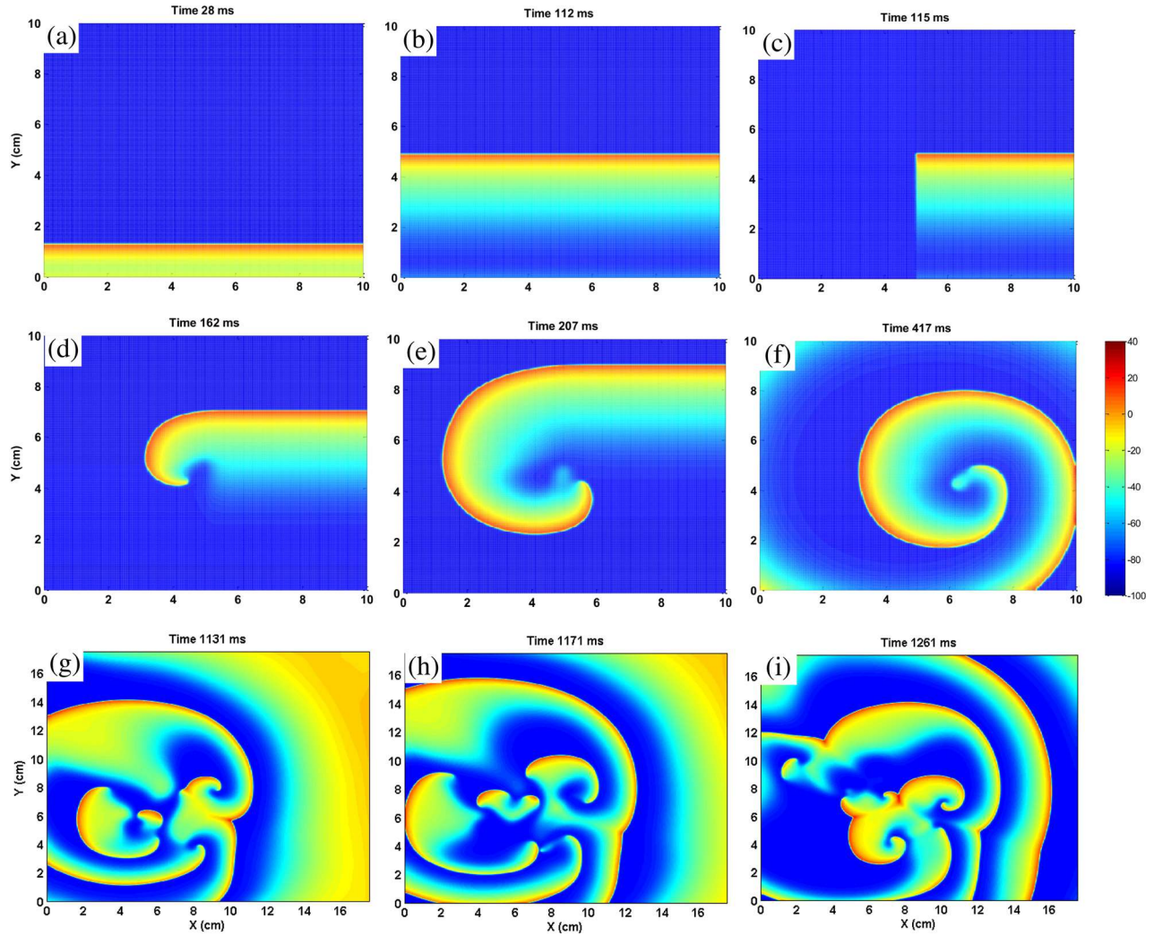
Fig. 10. Spiral wave evolution in the Beeler-Rueter model with speed-up calcium dynamics, calculated using the alternating direction implicit method: (a) initiation; (b) propagation; (c) symmetry break; (d) rotation begins; (e)–(f) spiral wave propagation. The domain size is 10 cm \times 10 cm, \Delta x = \Delta y = 0.025 cm, \Delta t = 0.01 ms. In panels (a)–(f), the spiral wave is shown for the first 500 ms; the times for each frame are indicated in the figure. Panels (g)–(i) show spiral wave breakup using the original parameters of the Beeler-Rueter model. Both the original and speed-up calcium parameters are given in Ref. 25. The domain size is 17.5 cm \times 17.5 cm.
