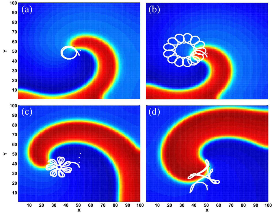
Fig. 4. Different types of spiral tip trajectories produced by changing the parameter \epsilon in the FitzHugh-Nagumo model: (a) \epsilon = 0.012 , (b) \epsilon = 0.010 , (c) \epsilon = 0.005 , and (d) \epsilon = 0.002 . Panel (a) shows a rigid rotation where the spiral shape remains constant and the tip of the spiral traces a circle. Panels (b)–(d) show more complicated flower-like patterns, called meandering spiral waves, with outward-facing petals.
