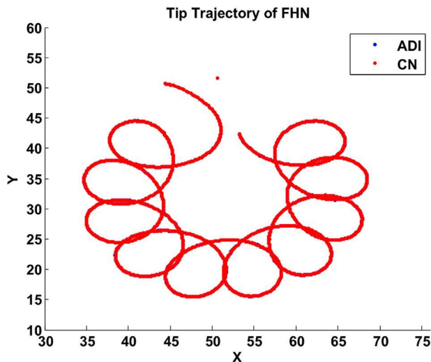
Fig. 11. The tip trajectory of the FitzHugh-Nagumo model using the same domain size, \Delta t , and \Delta x as in Fig. 3. The total time to generate this spiral is 2500 time units. The alternating direction implicit and the Crank-Nicolson methods produce almost identical trajectories.
